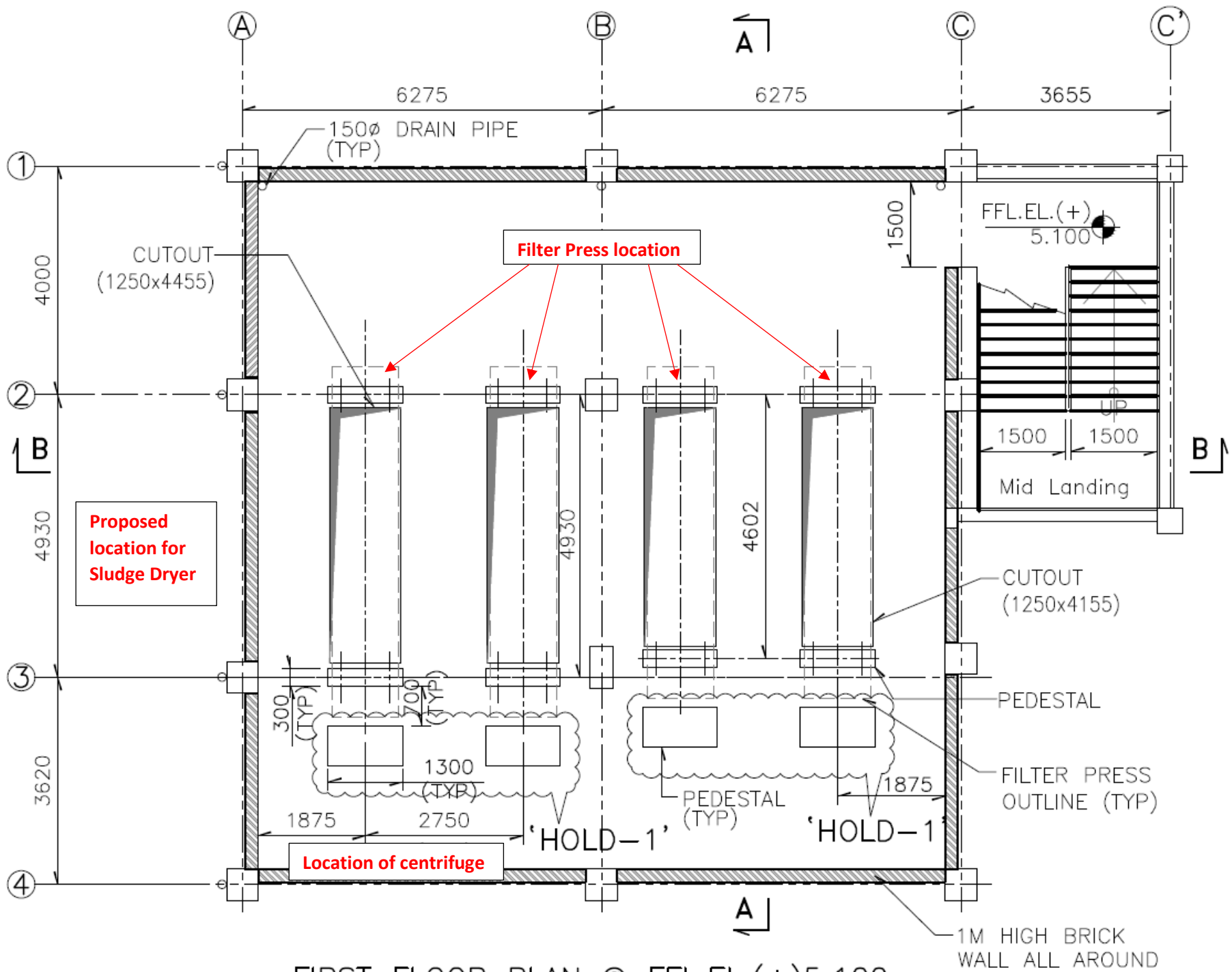
FIRST FLOOR PLAN @ FFL.EL.(+)5.100
