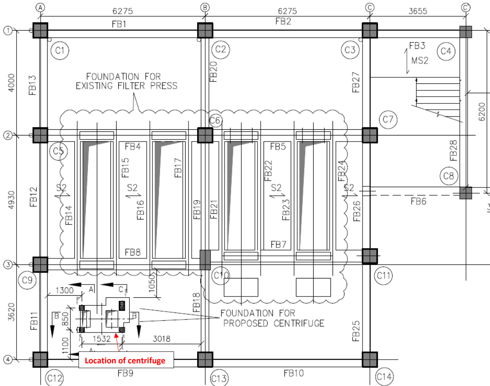
FLOOR PLAN AT TOC. @ EL.(+)742.025
